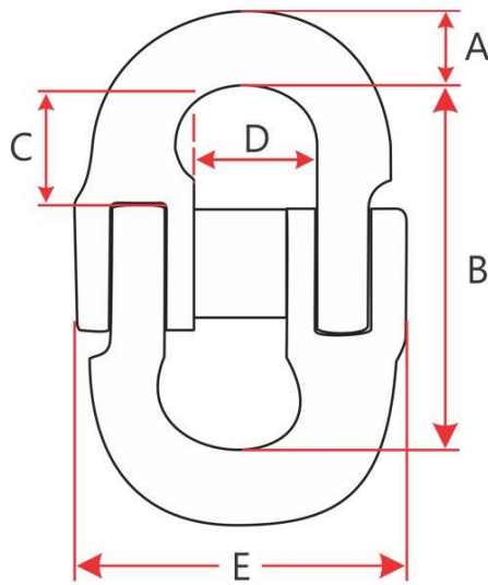
Connecting Link
