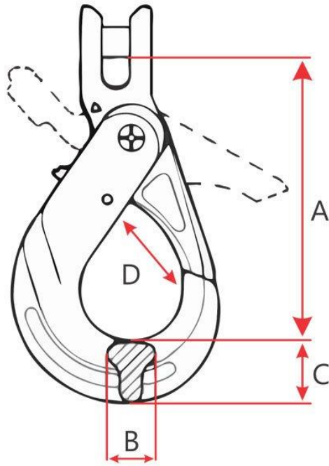
Clevis Type Self Locking Hook
