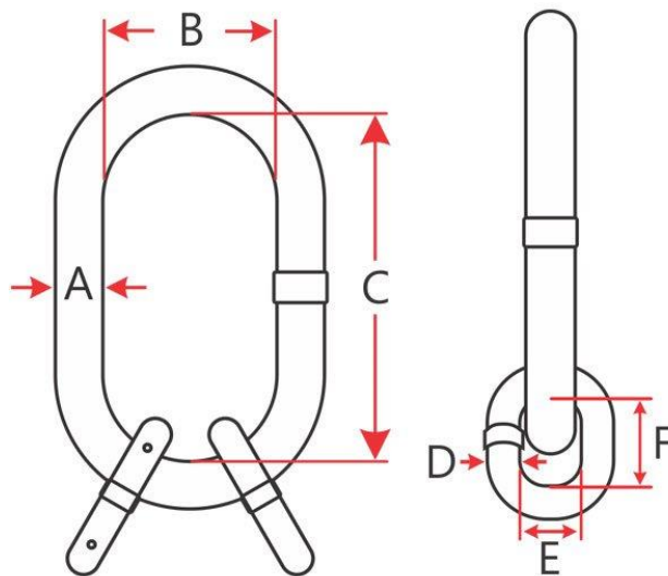
Sub Assembly
