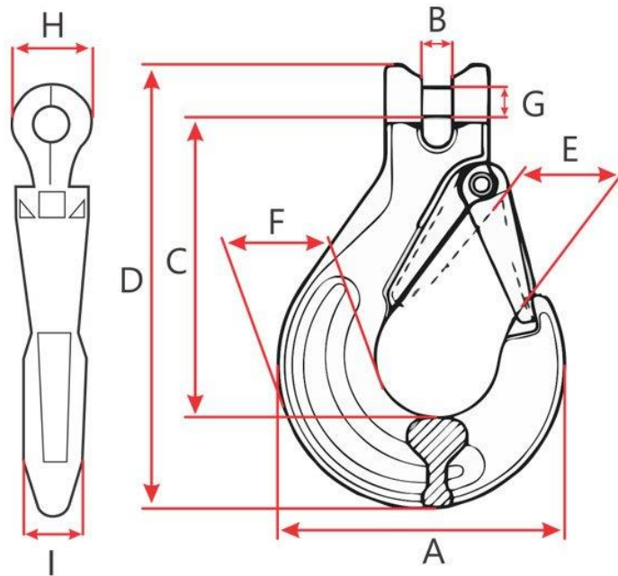
Clevis Type Safety Sling Hook
