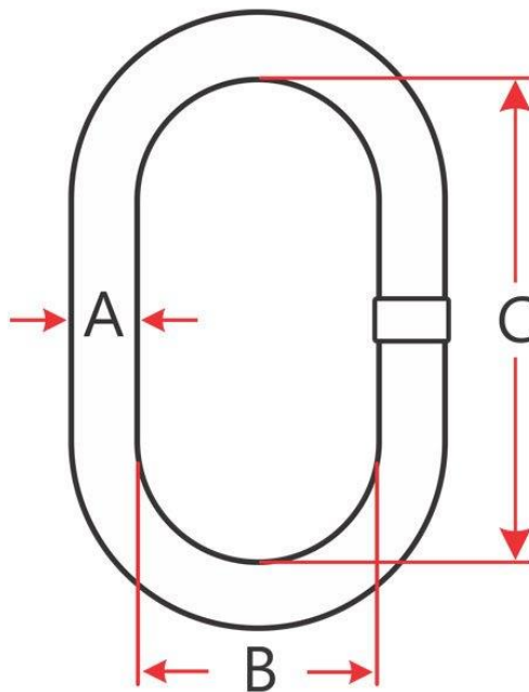
Master Link
