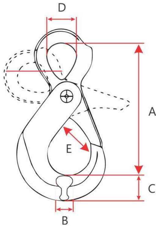
Eye Type Self Locking Hook
